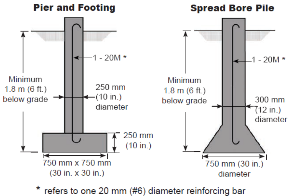
FIGURE 6 - Piles or piers
