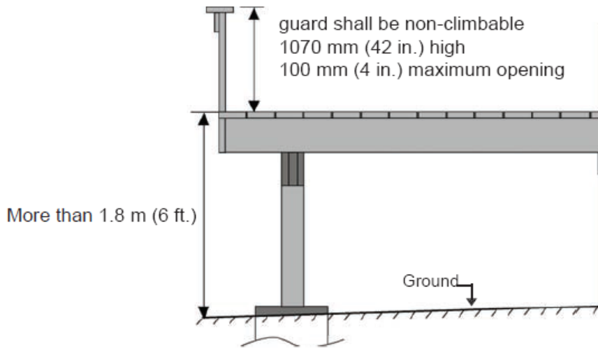
FIGURE 12 - Guardrail Height
