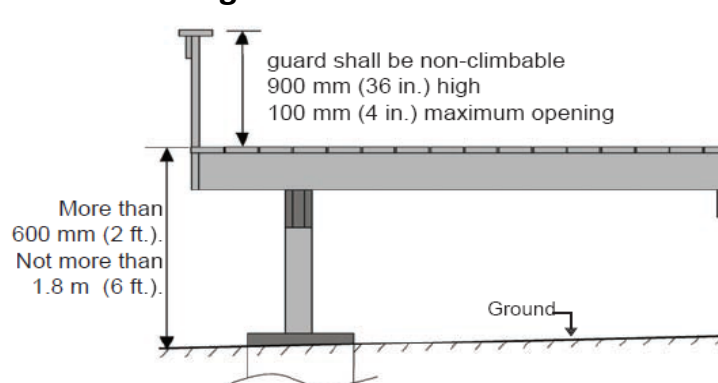
FIGURE 11 - Guardrail Height
