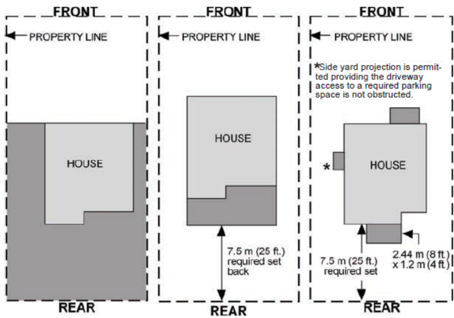
FIGURE 4 - Deck Location
