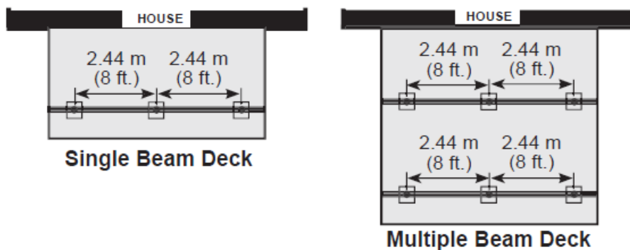
FIGURE 7 - Deck Beam Spacing
