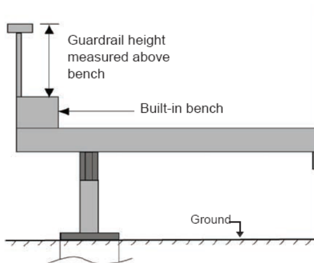
FIGURE 13 - Guardrail and Bench
