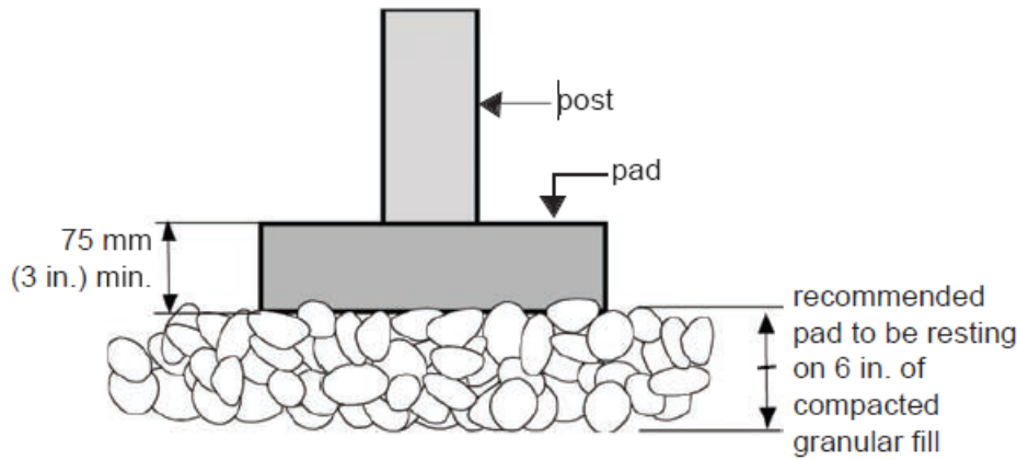
FIGURE 5 - Surface Pad Foundation
